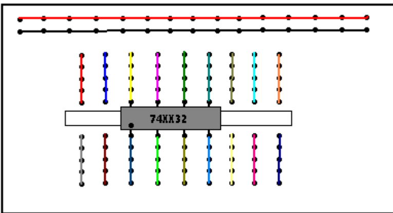
Fig. 5 Breadboard internal connections
