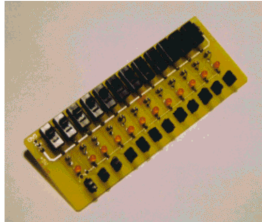
Fig. 1b Photo of the Switch PC Board
