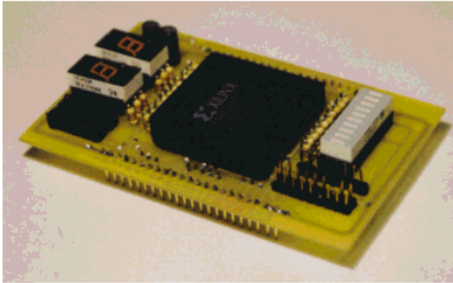
Fig. 1a Photo of the EVB2390 PC Board
