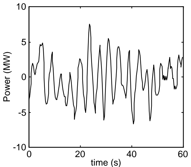
Figure 1. One minute of the power signal at BC Hydro Boundary from July 11, 1995, where the average value has been removed.
