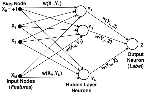
Fig. 1. The artificial neural network (ANN) in this work consists of inputs (features), hidden layer neurons, and an output neuron (label), connected through weighted edges. The weights, found through training, determine the function of the ANN.
