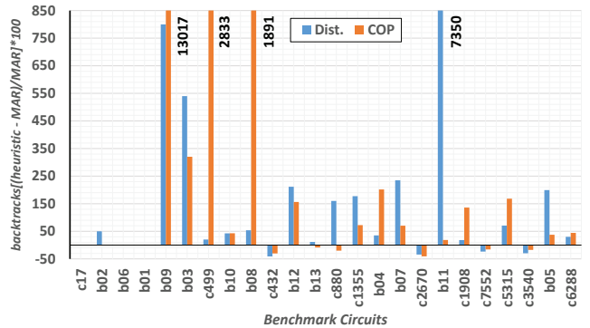
Fig. 6. When comparing the increase in backtracks when conventional heuristics are used for backtracing compared to an ANN, it is clear that using an ANN provides consistent and often substantial benefits. Positive bars indicate fewer backtracks by MAR over conventional heuristic.
