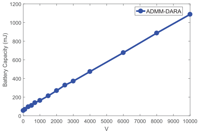
Fig. 7. Battery level vs. the control parameter V .
