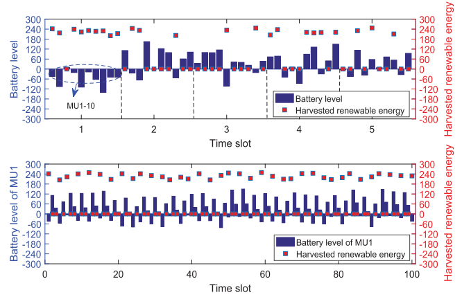
Fig. 5. Electricity charge/discharge over time ( V=1 ).
