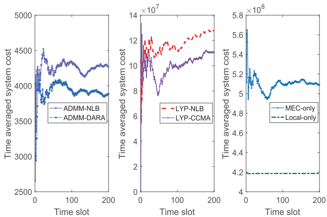
Fig. 8. Comparison of system performance (time averaged system cost) achieved by the six schemes.
