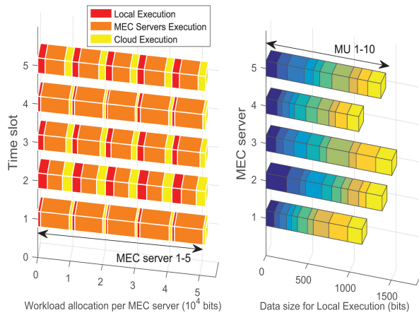
Fig. 4. The optimization of parallel offloading for multiple MEC servers and multi-users.
