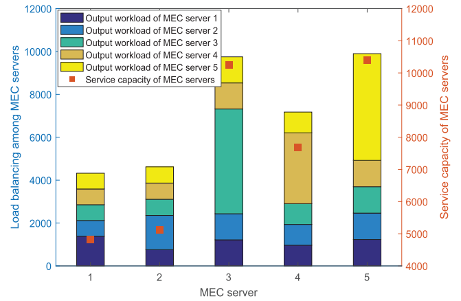
Fig. 2. Load balancing vs. service capacity of MEC servers when V = 1 .
