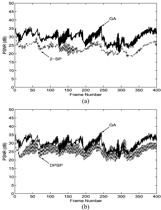
Fig. 9. PSNR curves of received video sequences. (a) GA-based algorithm versus 2-SP; (b) GA-based algorithm versus DPSP.
