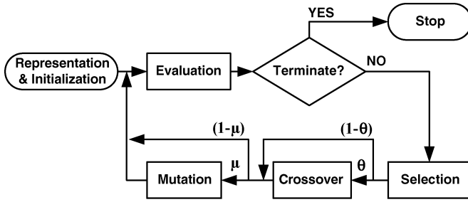
Fig. 4. Flow chart of the GA-based approach.
