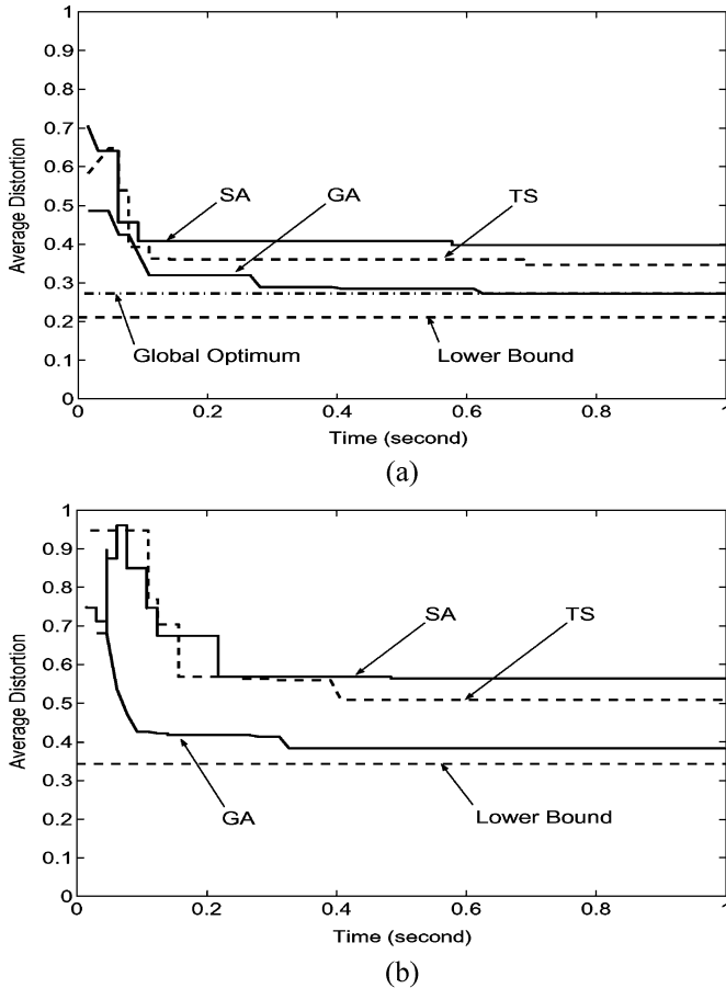
Fig. 8. Comparison of distortion evolution of three metaheuristic methods. (a) Distortion evolution for a 10-node network; (b) distortion evolution for a 50-node network.
