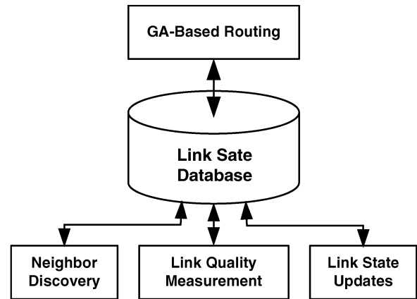
Fig. 10. Distributed implementation architecture for the GA-based multipath routing.
