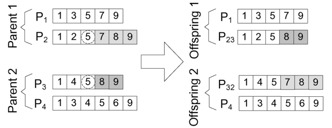
Fig. 6. Example of the crossover operation.
