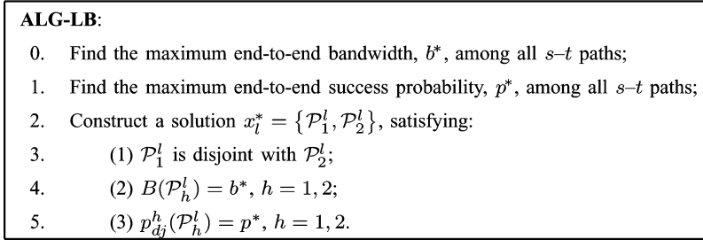
Fig. 3. A procedure to construct a lower bounding solution x_l^* .
