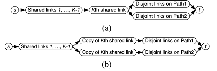
Fig. 2. The two solutions have the same set of links. The only difference between them is that a link is shared in \hat{x} (the K -th shared link), but not shared in \bar{x} (a copy of which is appended to each of the disjoint portions). (a) Solution \hat{x} ; (b) solution \bar{x} .
