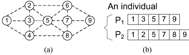
Fig. 5. Example network and coding of an individual ( s = 1 and t = 9 ). (a) Example ad hoc network; (b) example individual.
