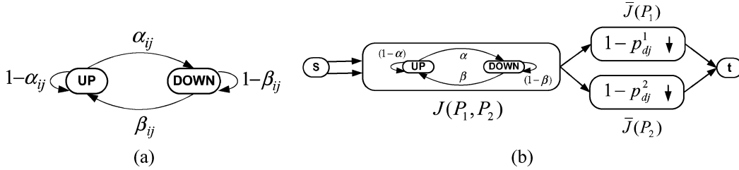
Fig. 1. Link and path models. (a) The Gilbert two-state link model; (b) a simplified path model for double-description video.
