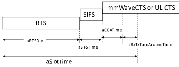
Fig. 6. The definition of aSlotTime in the proposed protocol.
