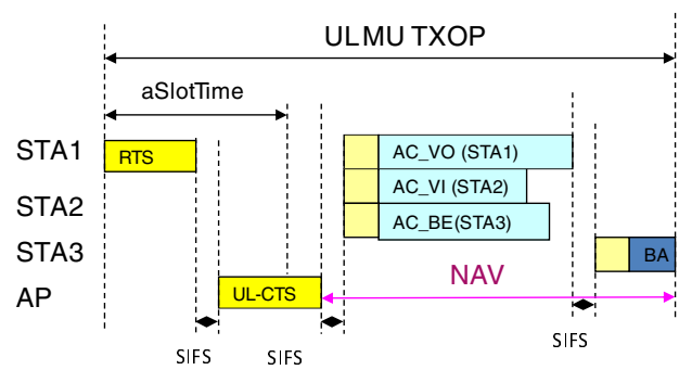
Fig. 4. UL MU operation.
