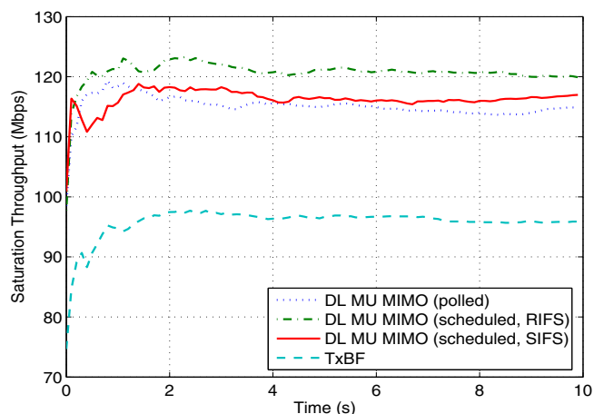
Fig. 11. Saturation Throughput S (with MAC protection).
