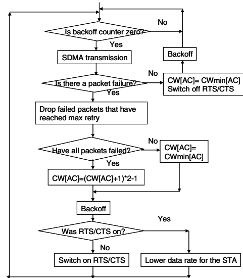
Fig. 4. Flow chart of the AP backoff procedure.
