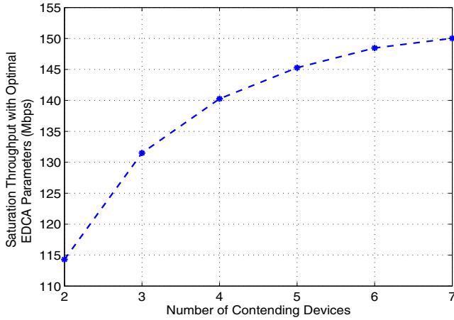
Fig. 8. Saturation throughput S vs. number of contending devices n (optimal EDCA parameters).
