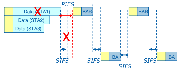
Fig. 3. Error recovery for polled response mechanism.
