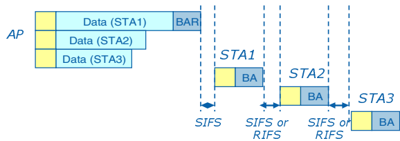
Fig. 2. CSMA/CA based DL MU MIMO protocol with scheduled response.
