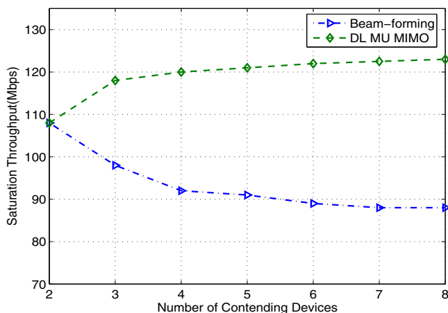
Fig. 9. Saturation throughput S vs number of contending devices n (bidirectional traffic).
