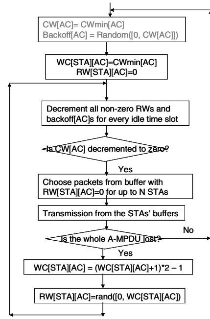
Fig. 7. Flow chart of weighted queuing.
