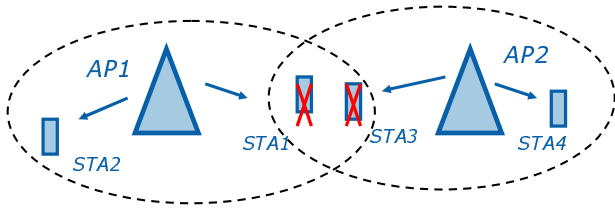
Fig. 5. Illustration of a hidden node scenario.
