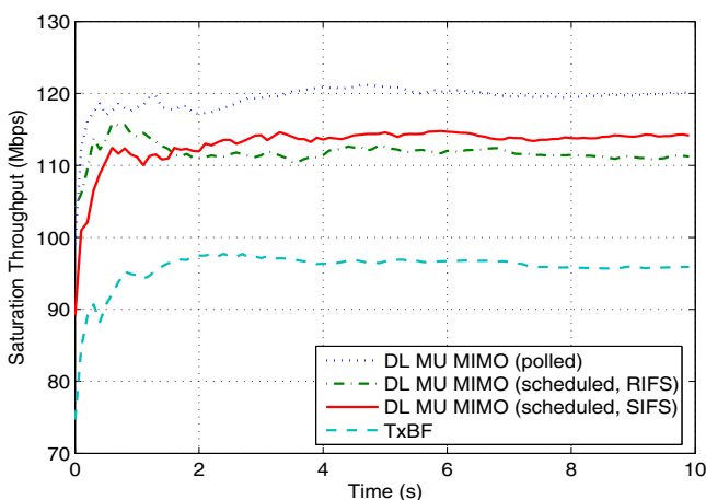
Fig. 10. Saturation throughput S (without MAC protection).
