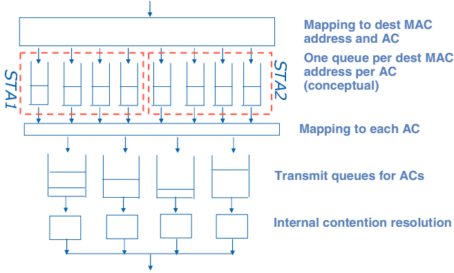
Fig. 6. Illustration of Weighted Queuing at the AP.
