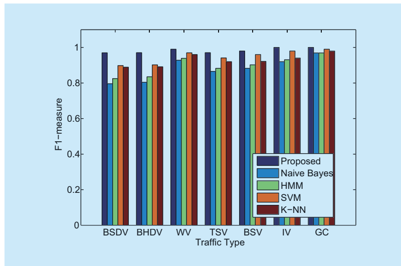
Fig. 4 Comparison of traffic classification methods in term of F1-measure
