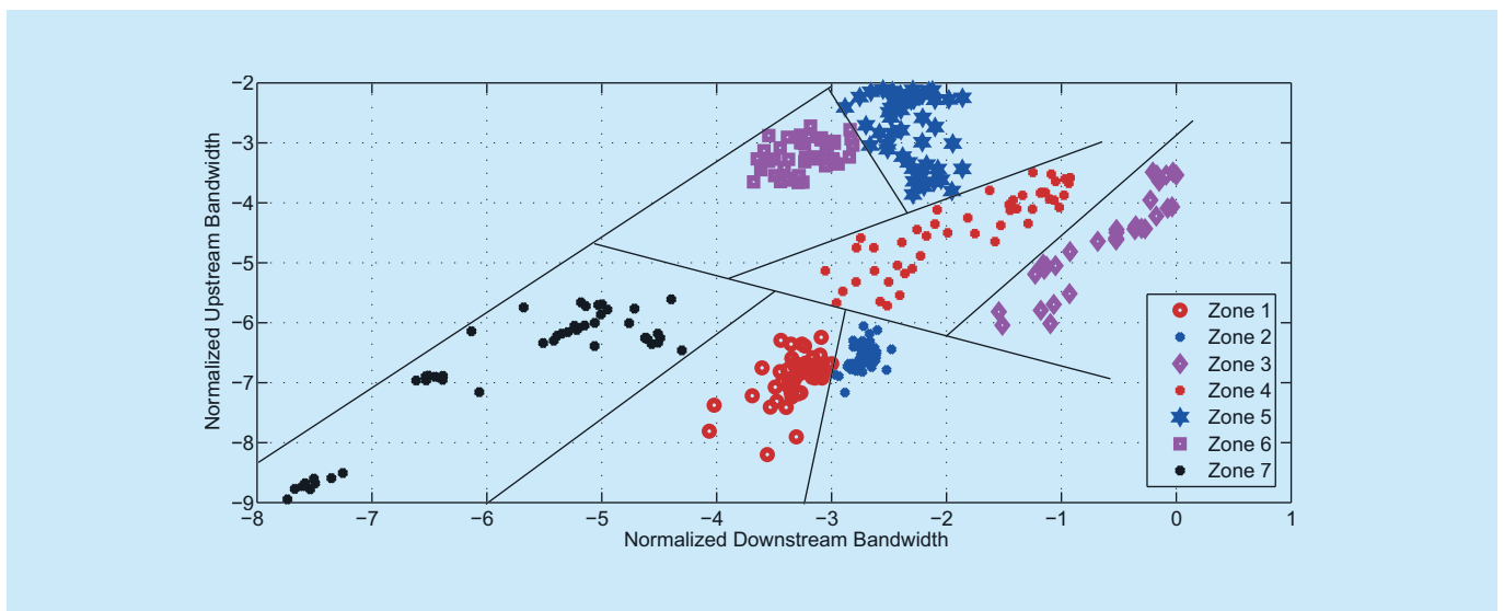
Fig. 2 The distributions of normalized logarithmic value of downstream/upstream rates (Mbps) for seven QoS categories
