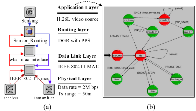
Fig. 4. H.26L Video Source Node Model.
