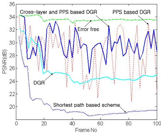
Fig. 5. Comparison of PSNR.
