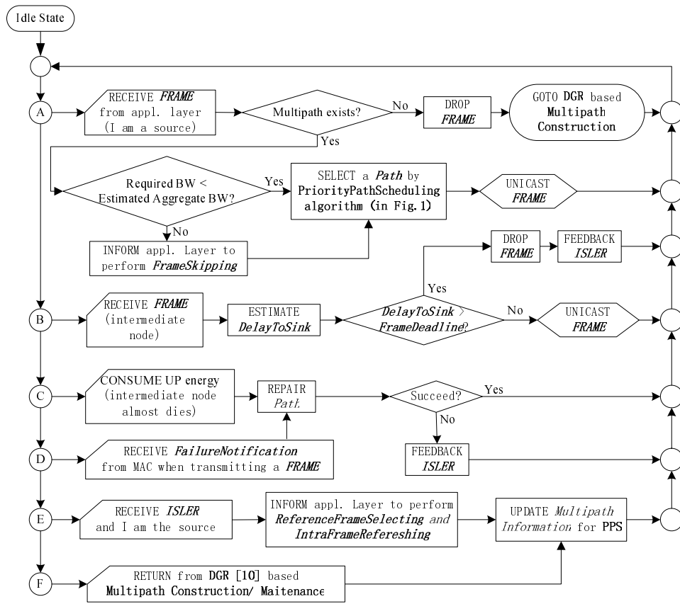
Fig. 3. Flowchart of joint PPS and cross-layer strategy.
