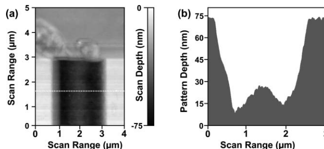
Fig. 3 AFM scan of the pattern imprinted into the PMMA resist: (a) top-view and (b) vertical cross-section at dashed line.
