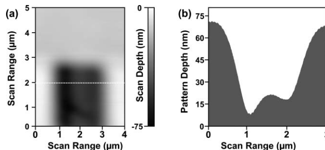
Fig. 4 AFM scan of the pattern transferred into Si substrate: (a) top-view and (b) vertical cross-section at the dashed line.
