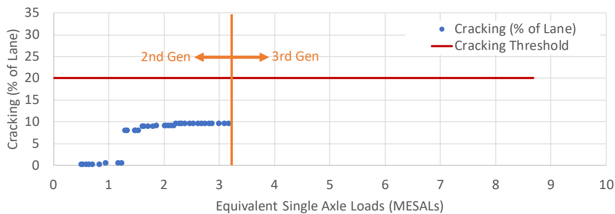
FIGURE 8 Percent cracking in the lane.
