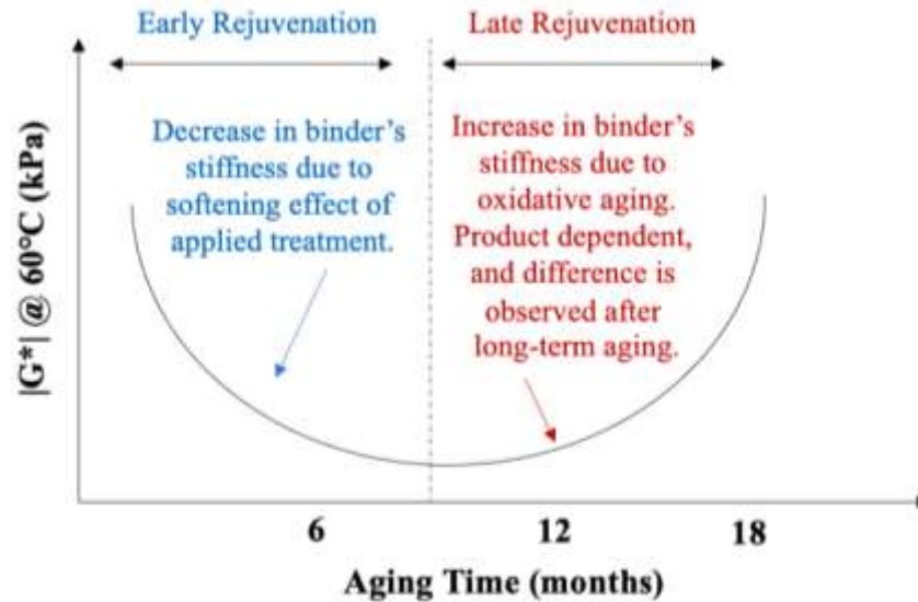
FIGURE 11 Hypothesized behavior of spray-on rejuvenator products.
