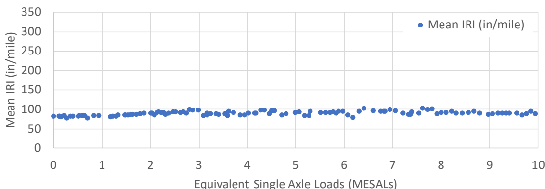
FIGURE 5 IRI results.
