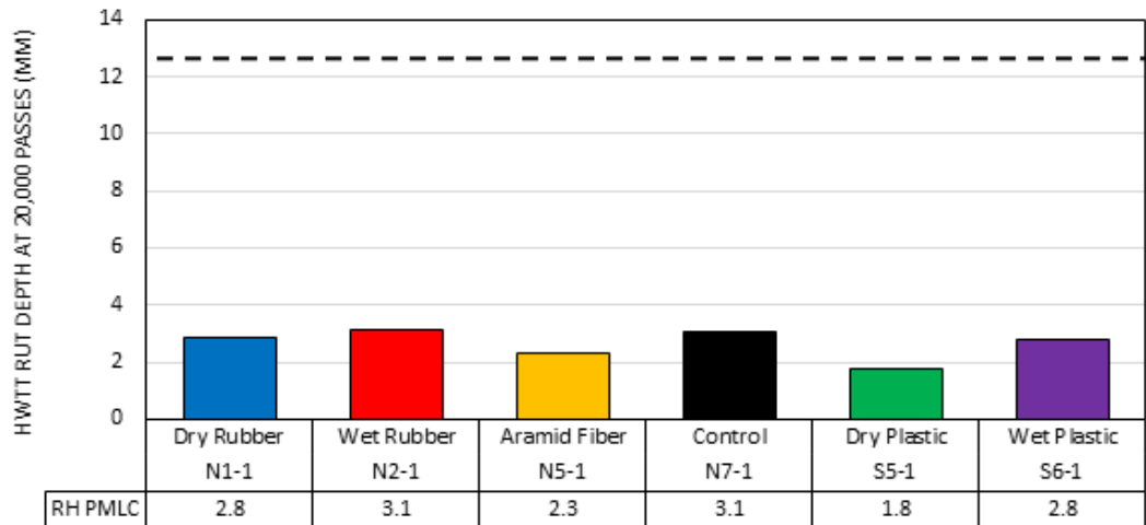
FIGURE 11 HWTT results for PMLC RH mixtures.
