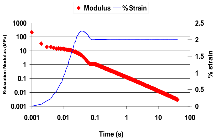
Figure 2. Example of time needed to reach constant strain for binder relaxation test (PG67-22 at 22°C).
