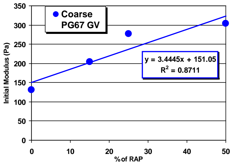
Figure 6. Linear relationship between initial modulus and percent of RAP (PG 67-22, 22°C).
