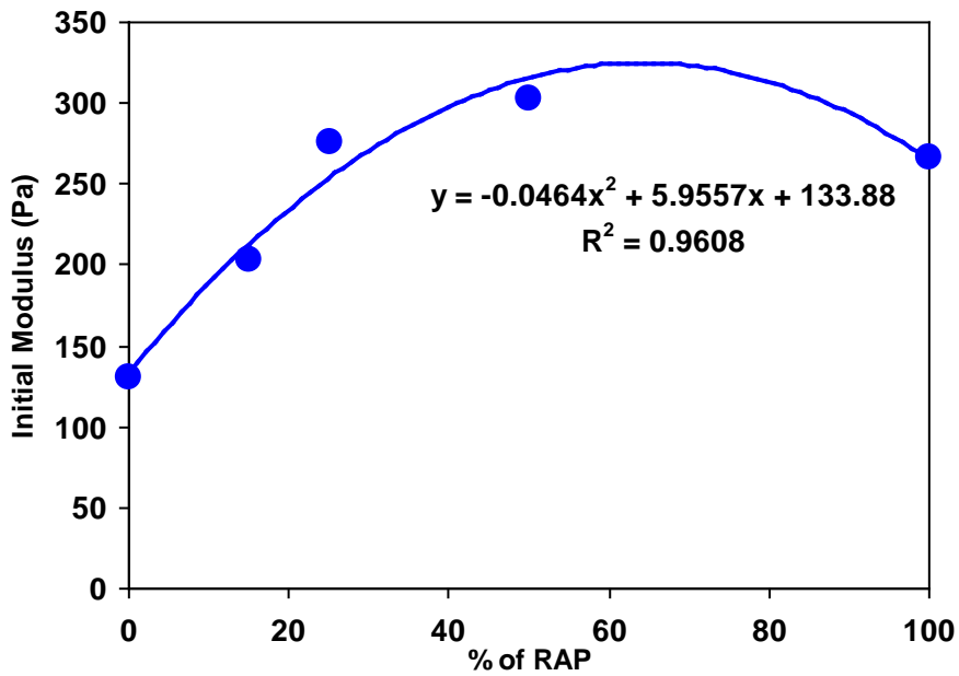
Figure 7a. Non-linear relation between percent of RAP and modulus (MN RAP, Gravel, PG 67-22, 22°C )
