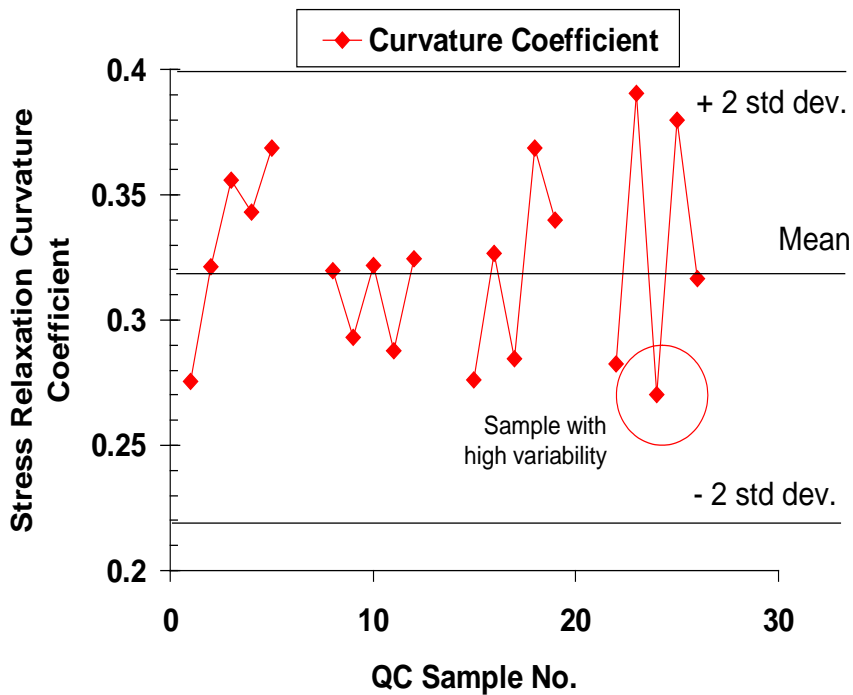
Figure 9. Coefficient of curvature process control chart for field study.
