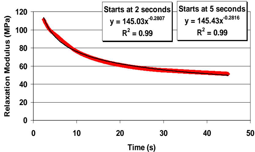
Figure 4. Typical relaxation curve and best fit curves.
