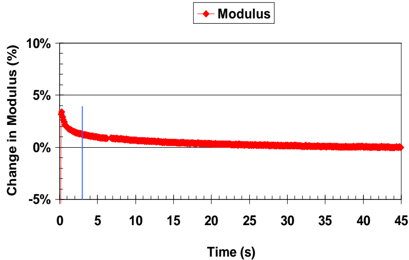
Figure 3. Setup time with steel cylinder in HMA stress relaxation equipment.
