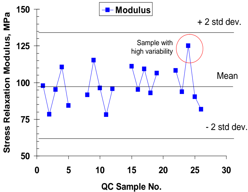
Figure 8. Stress relaxation modulus process control chart for field study.
