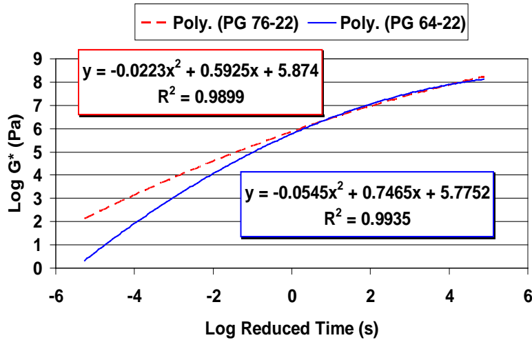
Figure 1. Binder G* master curves at 22°C.
