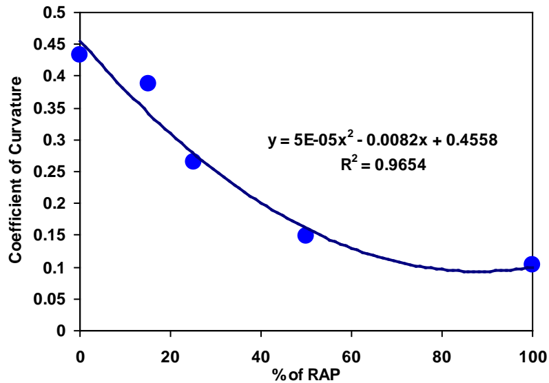
Figure 7b. Non-linear relation between percent of RAP and modulus (MN RAP, Gravel, PG 67-22, 22°C )
