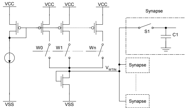
Fig. 6. Weight Control Circuit.
