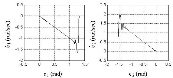
Figure 4: Behavior in the phase space
