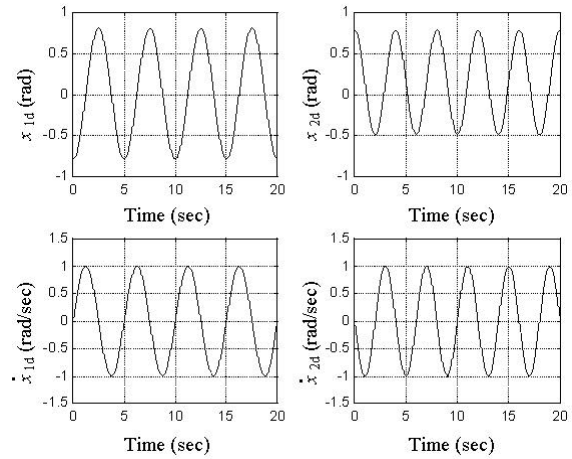
Figure 3: Reference state trajectories
