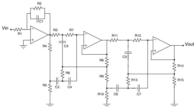
Fig. 4. Elliptic filter.
