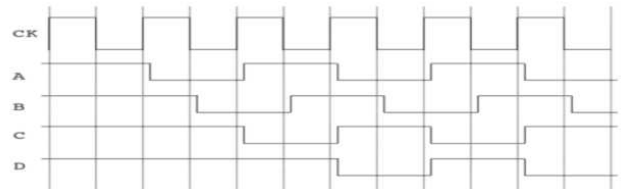
Fig. 16. Lockup latch in a scan chain.
