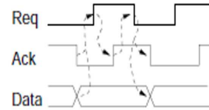
Fig. 5. A 4-phase bundled-data protocol.
