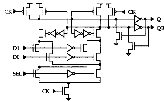
Fig. 6. DFF with embedded MUX2 logic (MUX2_DFF)
