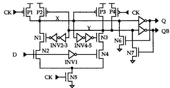
Fig. 5. Edge-triggered dual-rail dynamic flip-flop (DFF)
