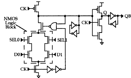
Fig. 4. SDFFF with embedded MUX2 logic (MUX2_SDFFF)
