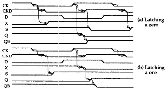
Fig. 2. Timing diagram for SDFFF
