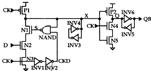
Fig. 1. Edge-triggered semi-dynamic flip-flop (SDFFF)
