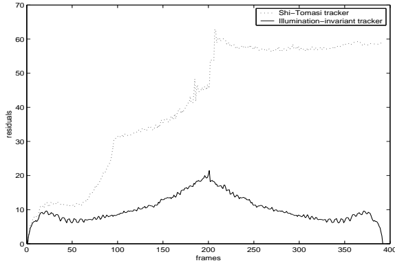
Figure 4. Evolution of SSD residuals. After 196 steps Shi-Tomasi tracker cannot compensate for changes in illumination. From frame 197 to frame 392 the box comes back to its original position and the patch can be matched exactly (i.e. the residual goes to zero) as expected.
