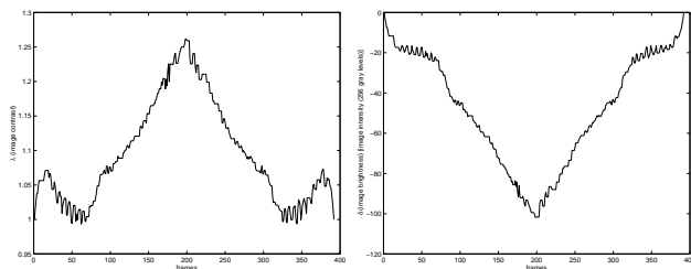
Figure 5. Left: Evolution of \lambda (image contrast). The image contrast increases until frame 197 and then goes back to 1 at frame 392, where the box returned to the original position. Right: Evolution of \delta (image brightness). The image brightness decreases until frame 197 and then increases going back to 0 where the patch returned to the original position.
