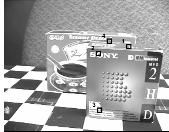
Figure 6. One snapshot from the “two boxes” sequence. In this sequence some features have been chosen using the selection algorithm of Shi-Tomasi. Feature 4 is chosen to show the behavior of the residual when there is partial occlusion. Feature 3 is an example of point feature that has high residual (when light changes are not accounted for) comparable to occluded features residual (see feature 4).
