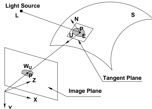
Figure 1. Image formation process when illumination is taken into account: the intensity value at p on the image plane depends in general on the light \mathcal{L} distribution, the observer position, the surface normal N at P and the albedo function E of S .
