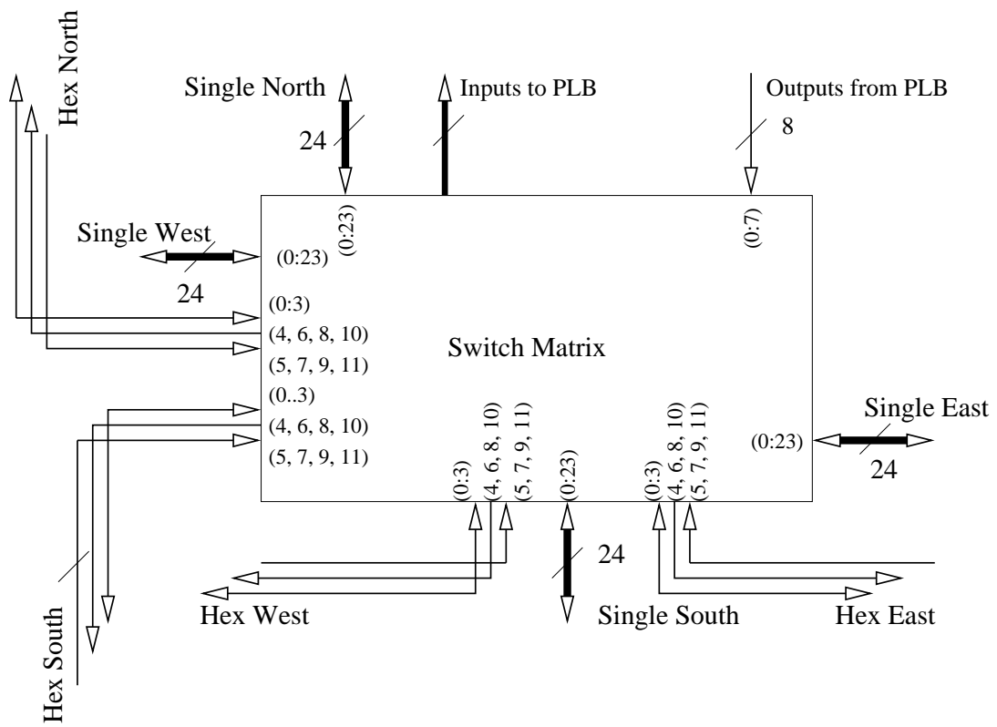
Figure 2.3: Switch Box CIP and Xilinx Interconnect Architecture
