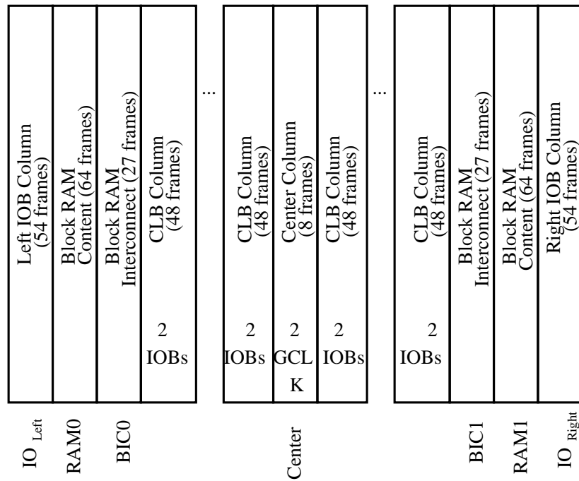
Figure 2.5: Xilinx Virtex-I and Spartan-II Addressing Scheme [Xil03d]
