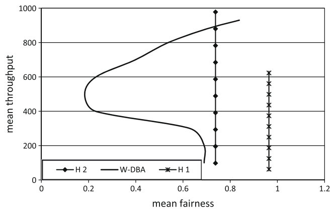
Fig. 6. Mean throughput and fairness for symmetric traffic at different offered load amounts where the point closest to the x-axis for each series is the lowest offered load.
