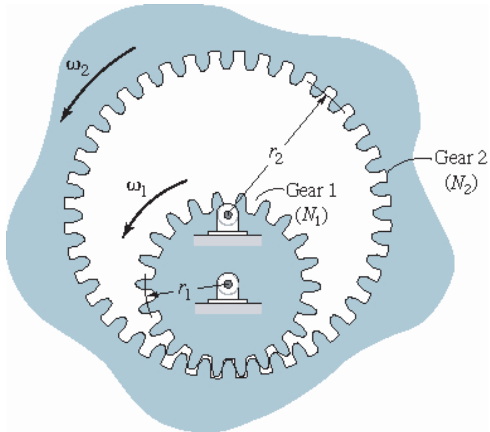
Internally Meshing Spur Gears
