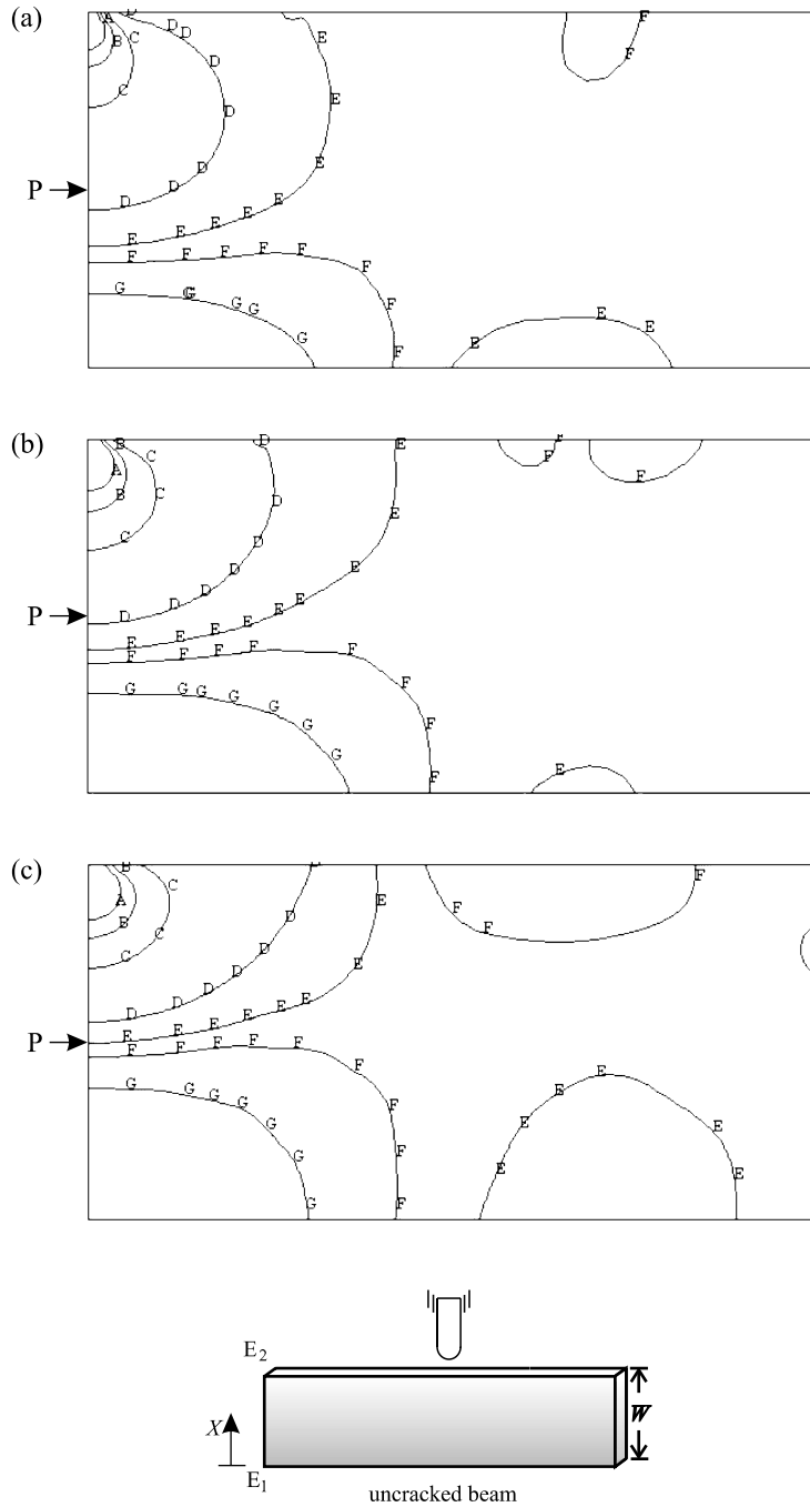
Fig. 13. (\sigma_x + \sigma_y) contours at non-dimensional time T = 5.7 . (A = -5, B = -3.5, C = -2, D = -0.5, E = -0.1, F = 0.1, G = 0.5) 10 MPa. (a) E_2/E_1 < 1 , (b) E_2/E_1 = 1 , (c) E_2/E_1 > 1 . Point P corresponds to (X/W = 0.5, y = 0) . Note that only the right-half of the beam is modeled.
