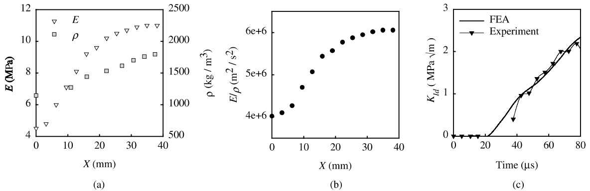
Fig. 5. Dynamic SIF history (c) for FGM shown in (a) and (b).
