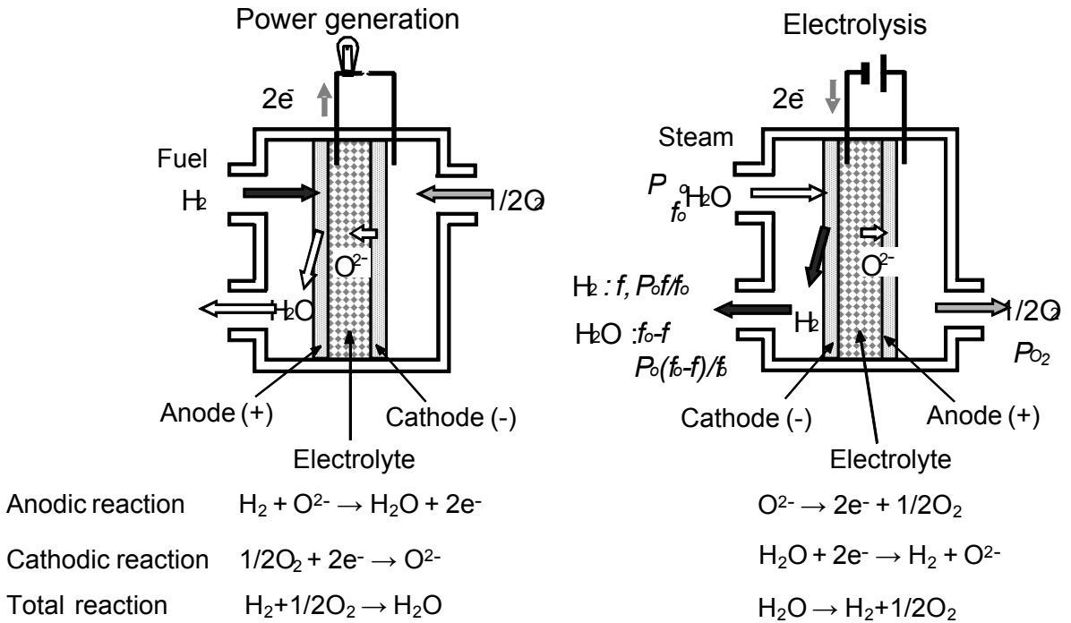
FIGURE 4.1 Principle of high-temperature electrolysis of steam (reverse reaction of SOFC)
