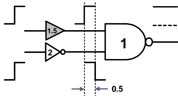
(c) Glitch elimination by path delay balancing
