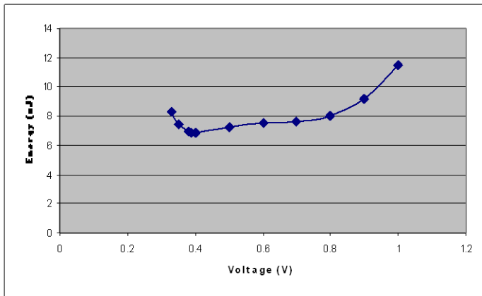
Fig. 4 plots the power x delay points given in Table 1 with respect to the voltage levels to find the optimum voltage point where we get the maximum energy savings for the flip flop.
