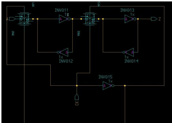
Fig. 3 shows the failure of the flip flop to drop to logic 0 at 0.42 V.
