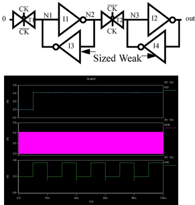
Fig. 2 (Top) shows the ratioed flip flop and (Bottom) shows the implementation in Design Architect.
