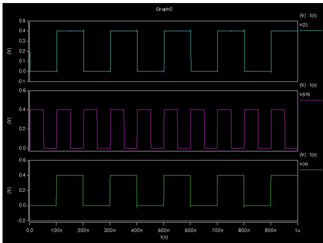
Fig. 5 shows the output of the flip flop when for the clocked signal of 0101 chain.
