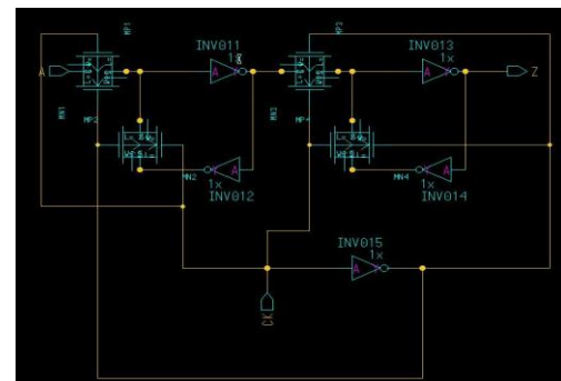
Fig. 1 [1] (Top) shows the implemented flip flop and Fig. 2 (Bottom) shows the corresponding schematic in Design Architect.
