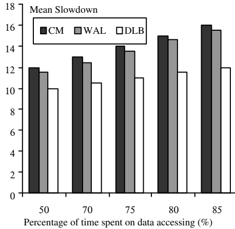
Fig. 3. Mean slowdowns as a function of the percentage of time spent on data accessing.
