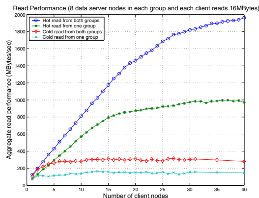
Figure 3. Read performance in the cases of cold read and hot read, as a function of the number of client nodes.
