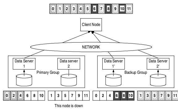
Figure 5. Skipping the heavily loaded data server nodes and reading the data from their mirroring server nodes.
