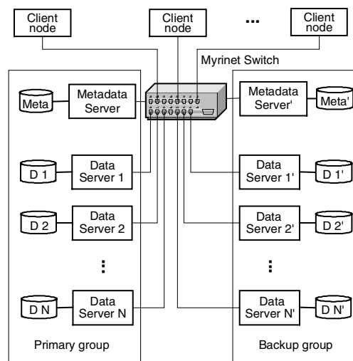
Figure 1. Block Diagram of CEFT-PVFS.
