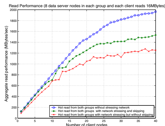
Figure 7. Hot read performance improvement by skipping the server with heavy network load and reading the data from its mirror.
