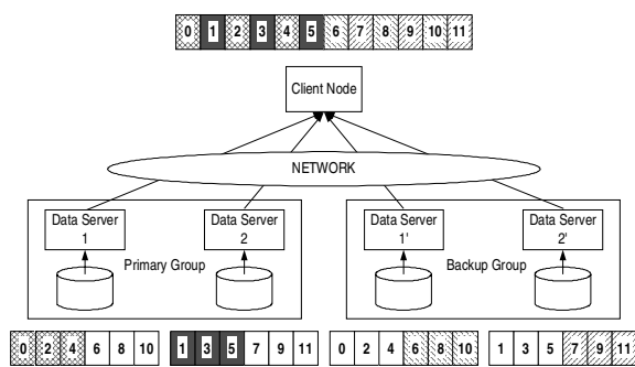
Figure 2. Reading interleaved data from both groups, half from the primary group, and half from the backup group.
