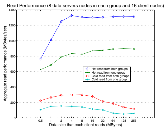
Figure 4. Read performance of cold read and hot read as a function of data size that each client reads.
