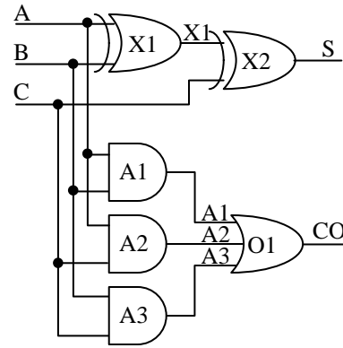
Figure 2. Completely specified logic diagram for full adder circuit.
