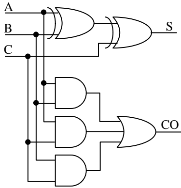
Figure 1. Logic diagram for full adder circuit.
