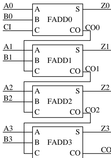
Figure 4. 4-bit adder constructed from 4 full adders.
