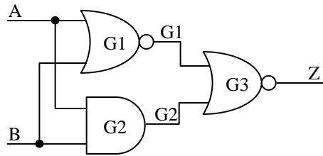
Figure 3. Logic diagram for elementary logic gate representation of an exclusive-OR.
