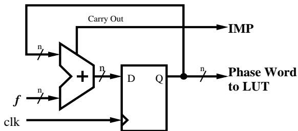
Fig. 6. Proposed IMP Circuit for Frequency Response Measurement.
