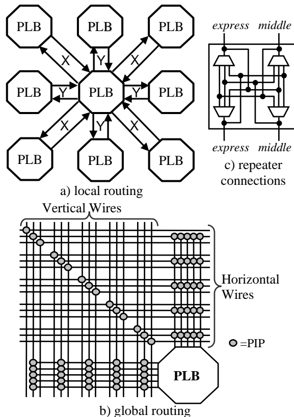
Figure 3. Routing resources
