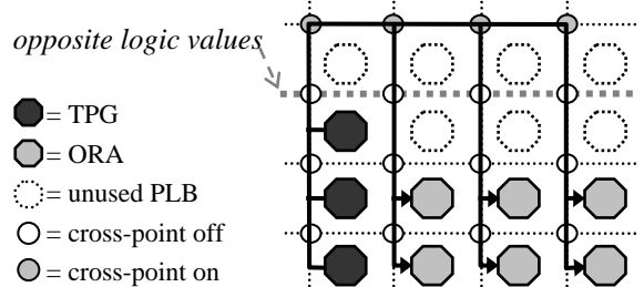
Figure 8. Routing BIST for cross-point PIPs
