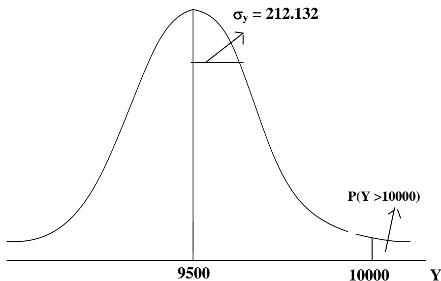
Figure 4. The approximate pdf of Y
