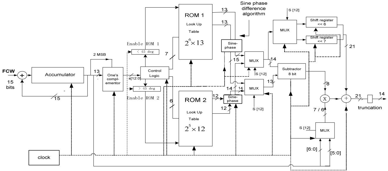
Figure 2. Phase to sine amplitude conversion architecture using non-linear addressing.
