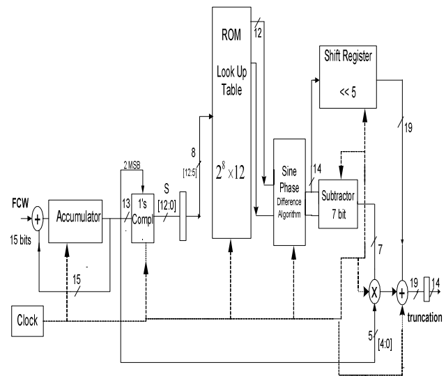
Figure 1. Phase to amplitude conversion using a multiplier.
