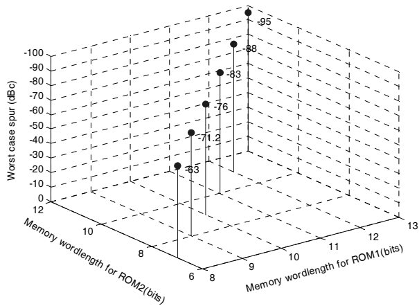
Figure 3. ROM word length vs. worst-case spurs for nonlinear addressing.
