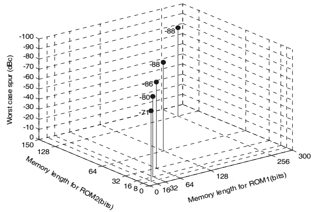
Figure 4. ROM length vs. worst-case spurs for nonlinear addressing.
