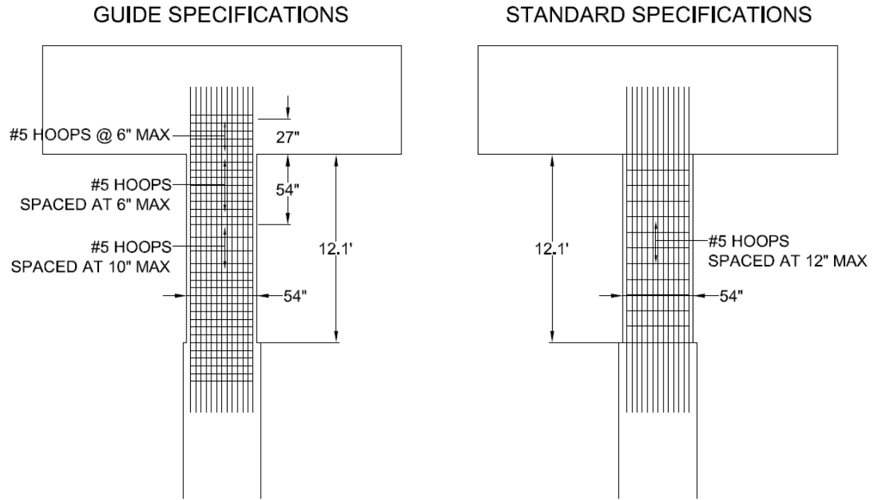
Figure 4.27: Little Bear Creek Bridge Bent 2 Final Design Details
