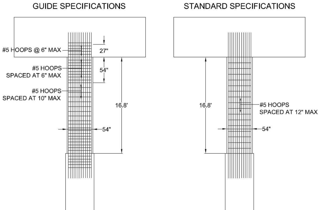
Figure 4.27: Little Bear Creek Bridge Bent 2 Final Design Details
