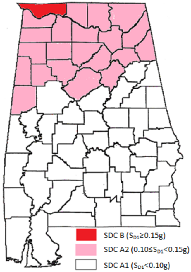
Figure 4.3: Alabama SDC Map for Soil Site Class C
