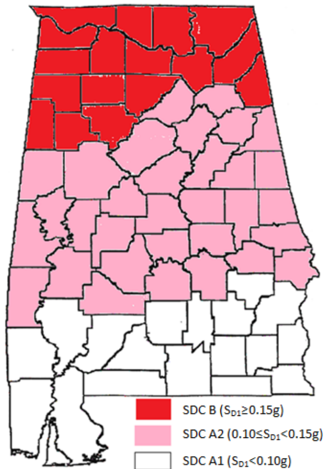
Figure 4.4: Alabama SDC Map for Soil Site Class D
