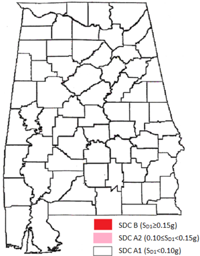
Figure 4.2: Alabama SDC Map for Soil Site Class B
