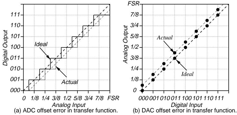
Figure 10.8: Offset error in ADC (a) and DAC (b) transfer functions.
