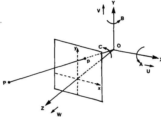
FIG. 1. Coordinate system.
