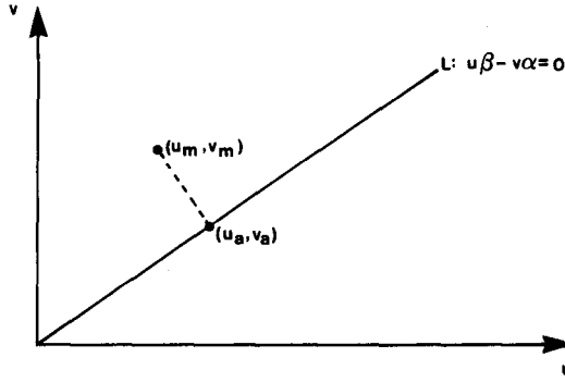
FIG. 2. Geometrical interpretation.
